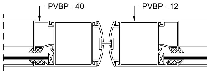
BP29 Remate inf. travessa porta
